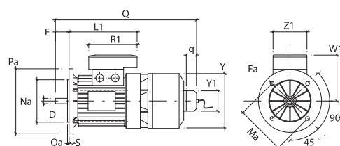
BAE B14
