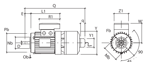
BAE 160/180/200/225 B3
