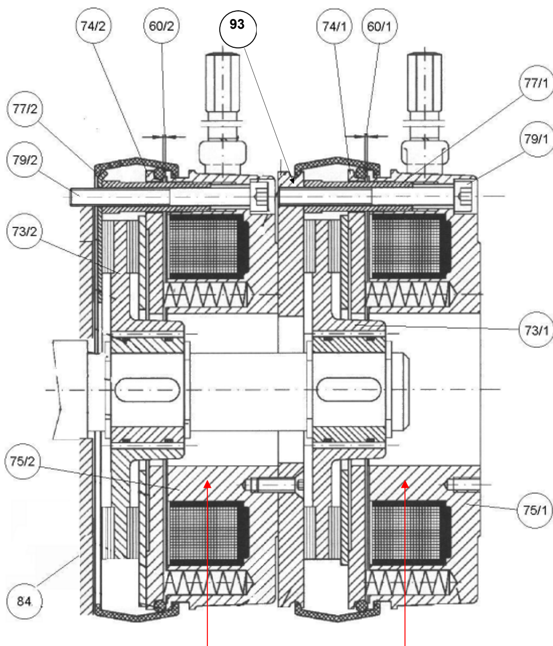
Brake assembly 2
