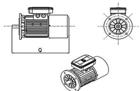
BMAV Series
