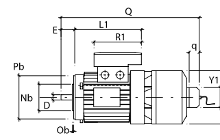
BAE 160/180/200/225 B3
