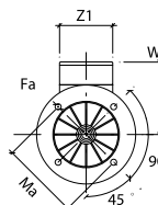
BAE B14
