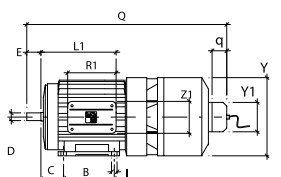
BAE 160/180/200/225 B3
